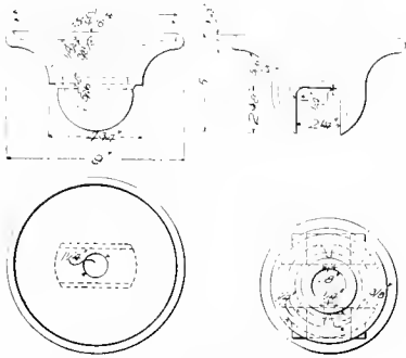
Figs. 4864-66. EQUALIZING-BAR SPRING-SEAT.
